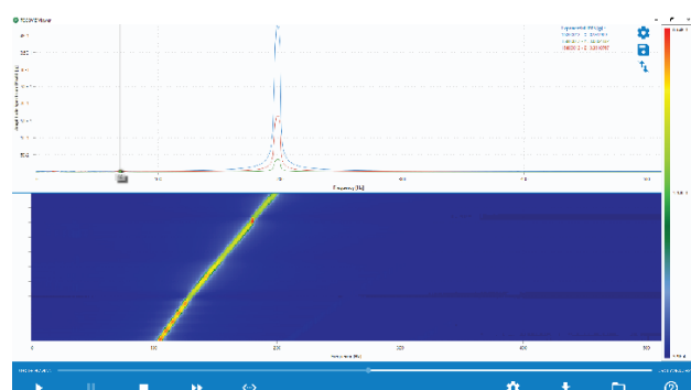
谱图特征 Recovib_FEEL_EN-Rev1p0
